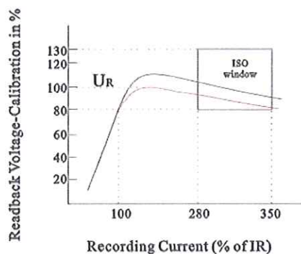
Saturation Curve
